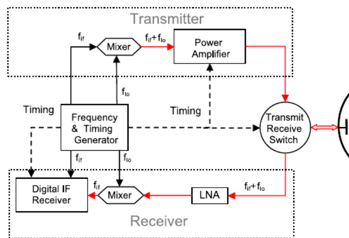
Fig. 2: Simplified Block Diagram of RWP
