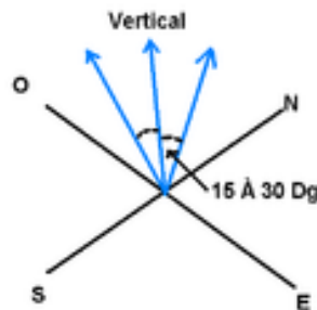
Fig. 1: Orientation of Beams In Wind Profiler
